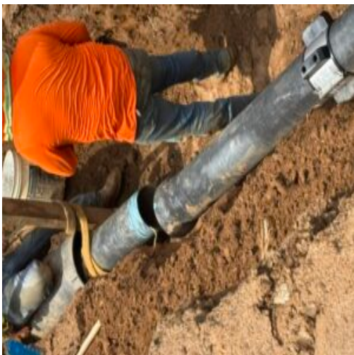
Pushing 8" ductile iron pipe through 16" steel casing
