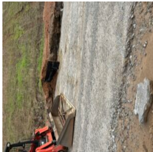
Sub base prep. and check dam installations
