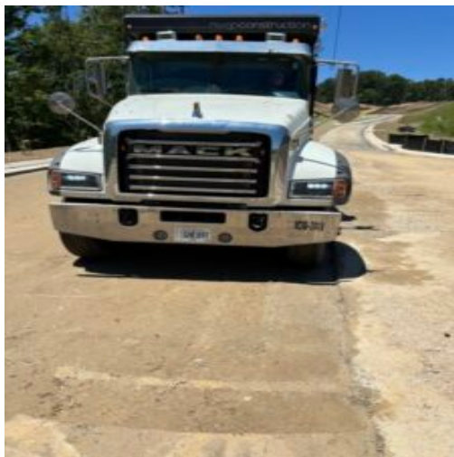
Proof rolling subbase stone at Nature Walk Pkwy. between sanitary sewer manholes #9 and 11 using a tandem dump truck with 19 tons.
