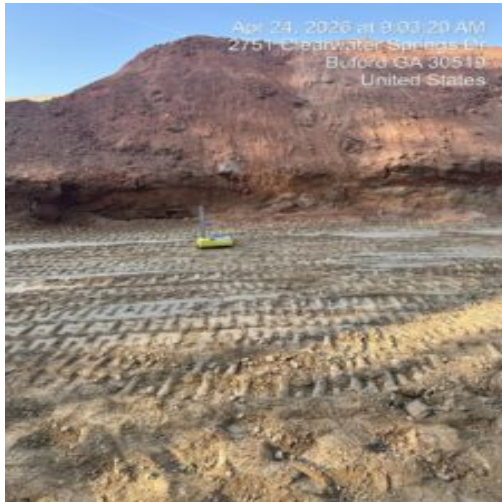
performing density testing with nuclear guage.
