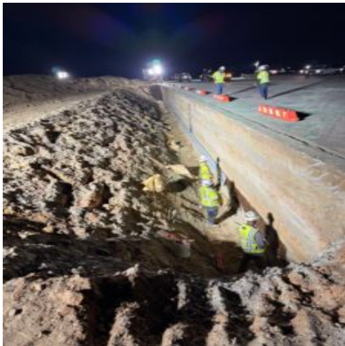
Waterproof membrane being installed
