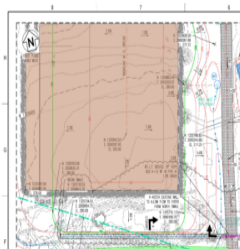
Highlighted region shows the fill material placement
