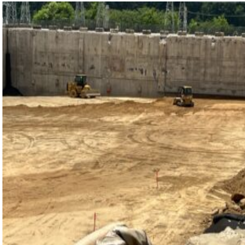
Backfill being placed as lift 8 in the Section 2 area
