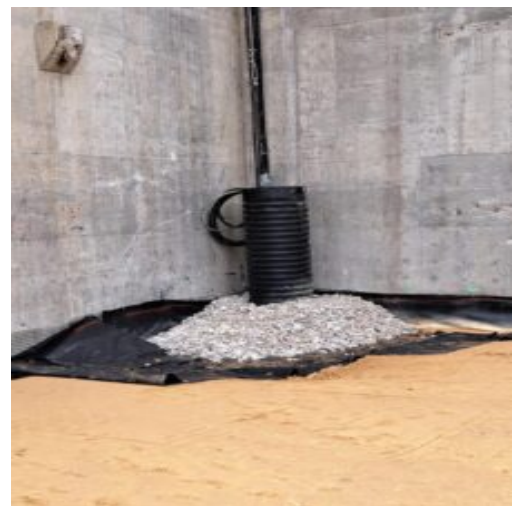
Placement of 24B Stone
