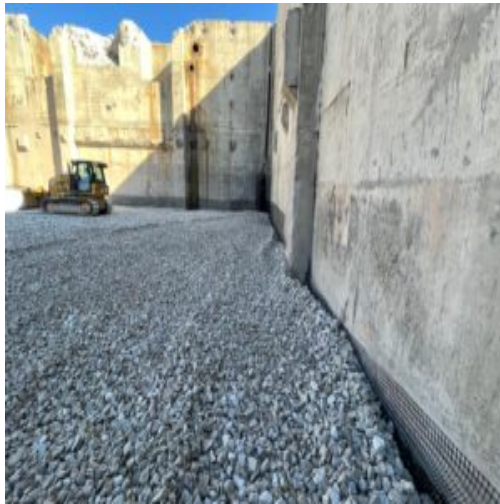
This is placement of # 24 stone as seen facing bakers creek wall.
